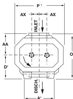
Horizontal configuration (Vertical air flow)
